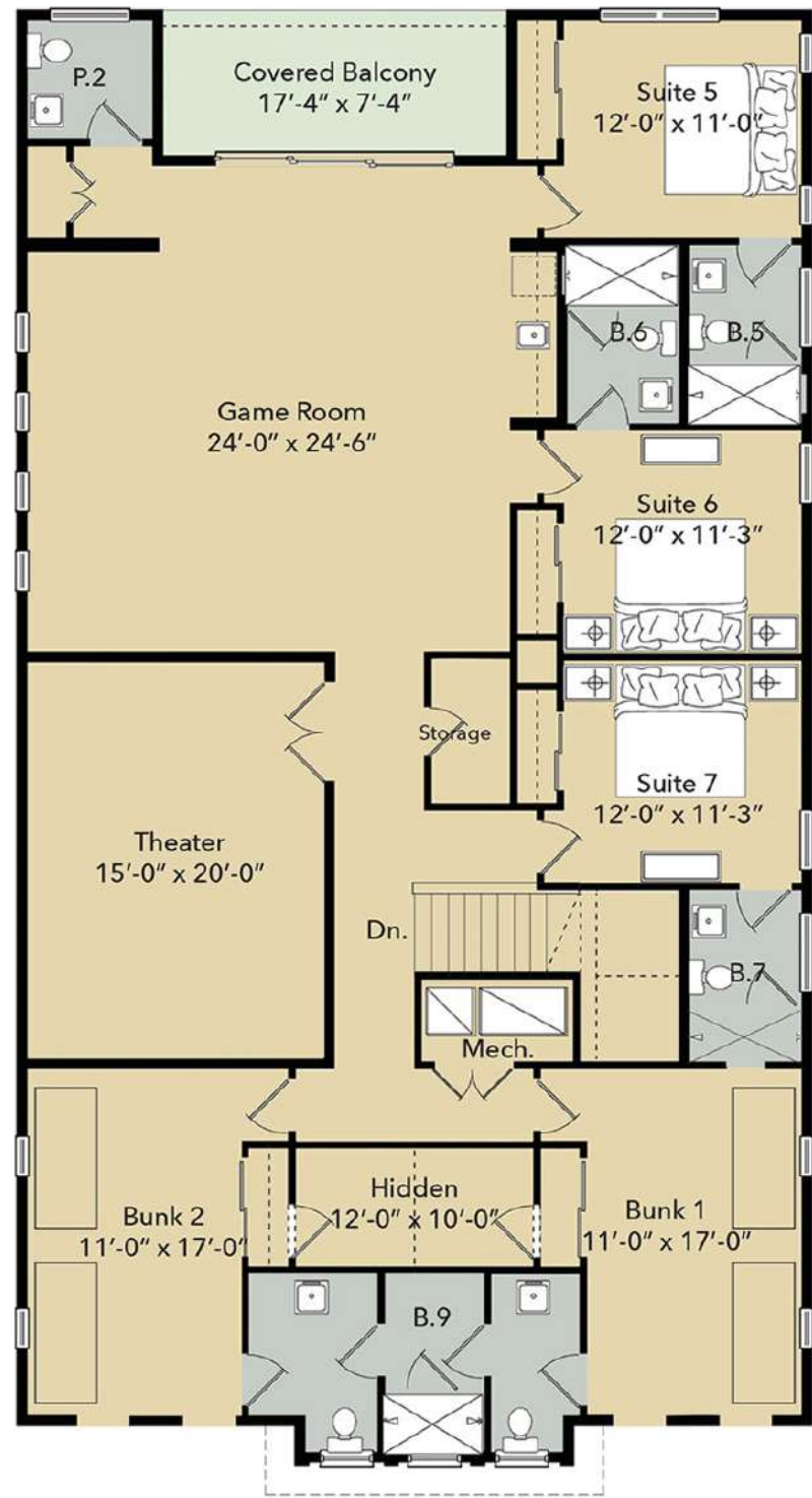
SECOND FLOOR
