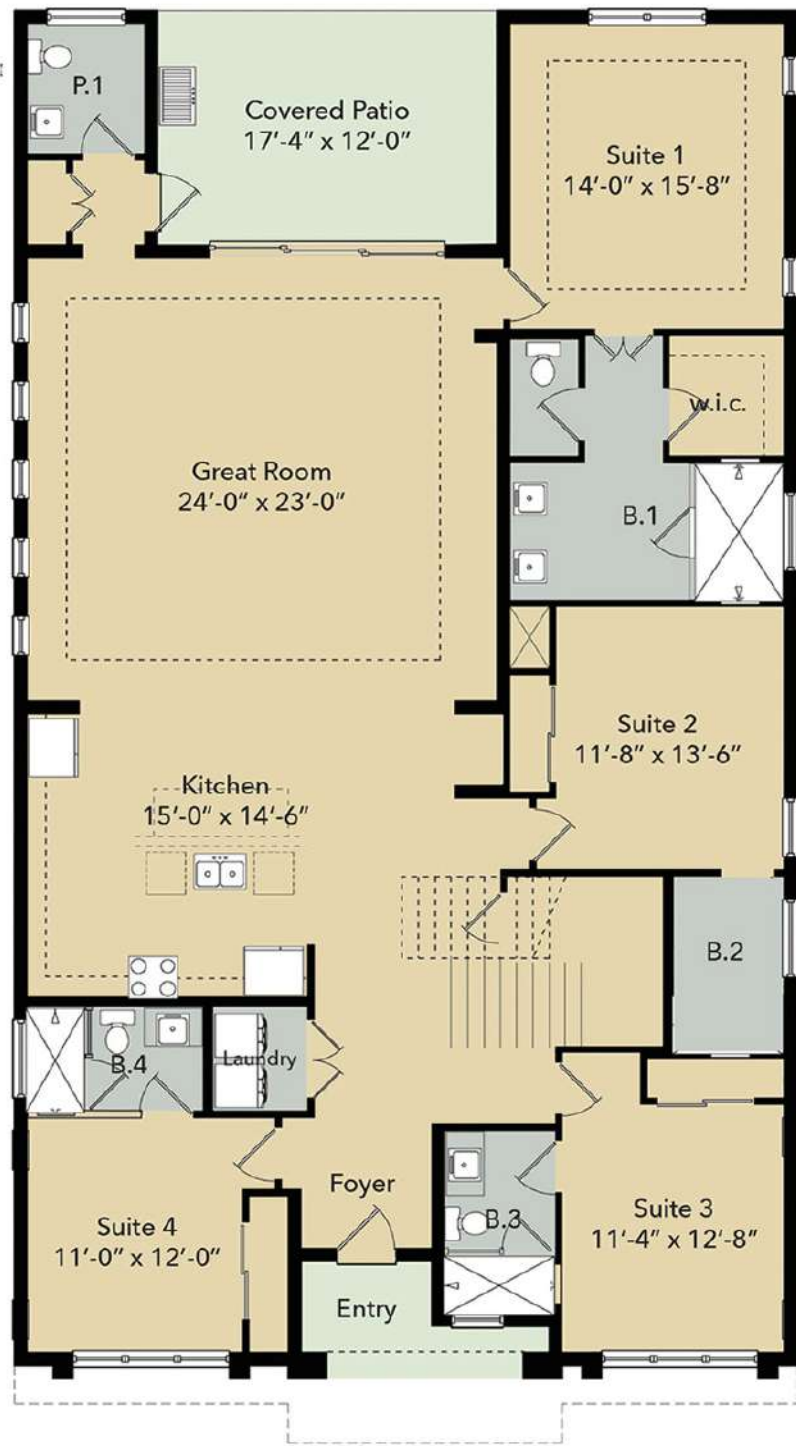
FIRST FLOOR
